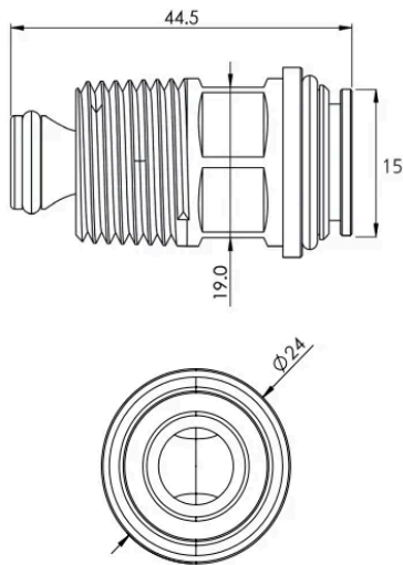
Manual Shut Off Valve
