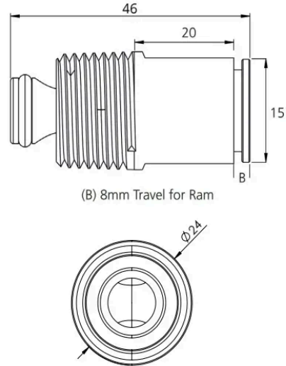
TRV Shut Off Valve
