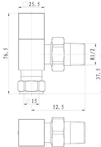
Angled Square Valve
