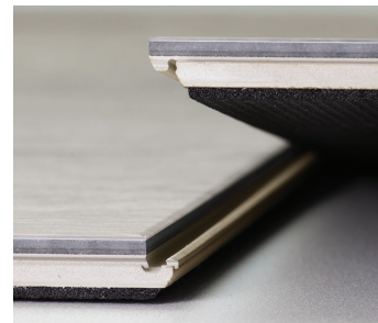
PVC Wide Panel shown in Grey Marble
